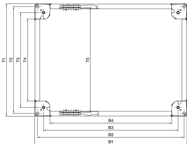
Dimensional drawing base/plinth 100 mm high
