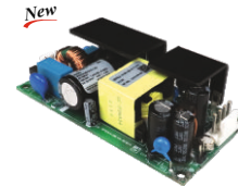
OPS2x4-60 101.6(L) X 50.8(W) x 30(H)mm
